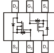
TOP VIEW Schematic and Transistor Diagram
